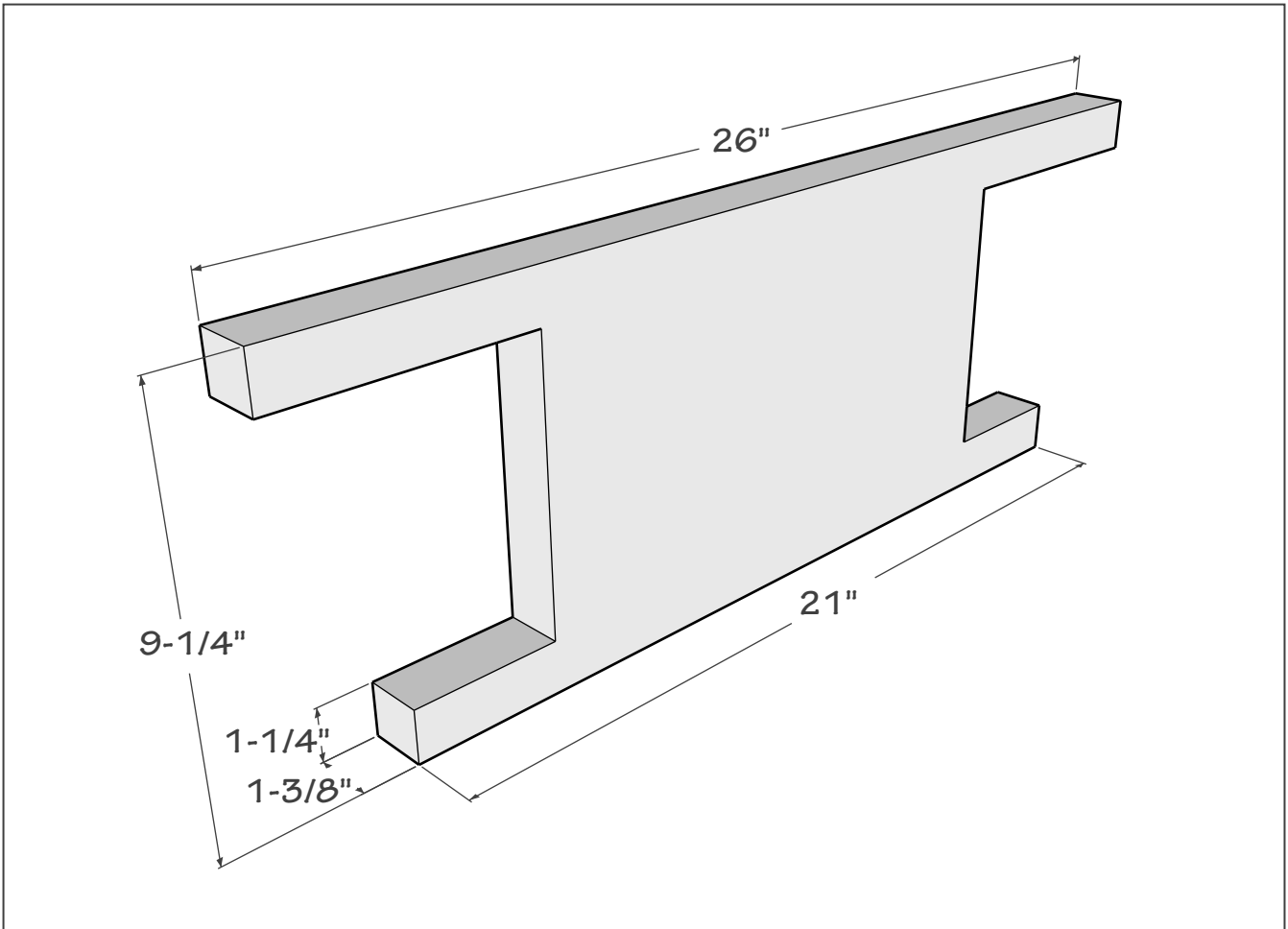
Seat drilling jig, made from 2x material
