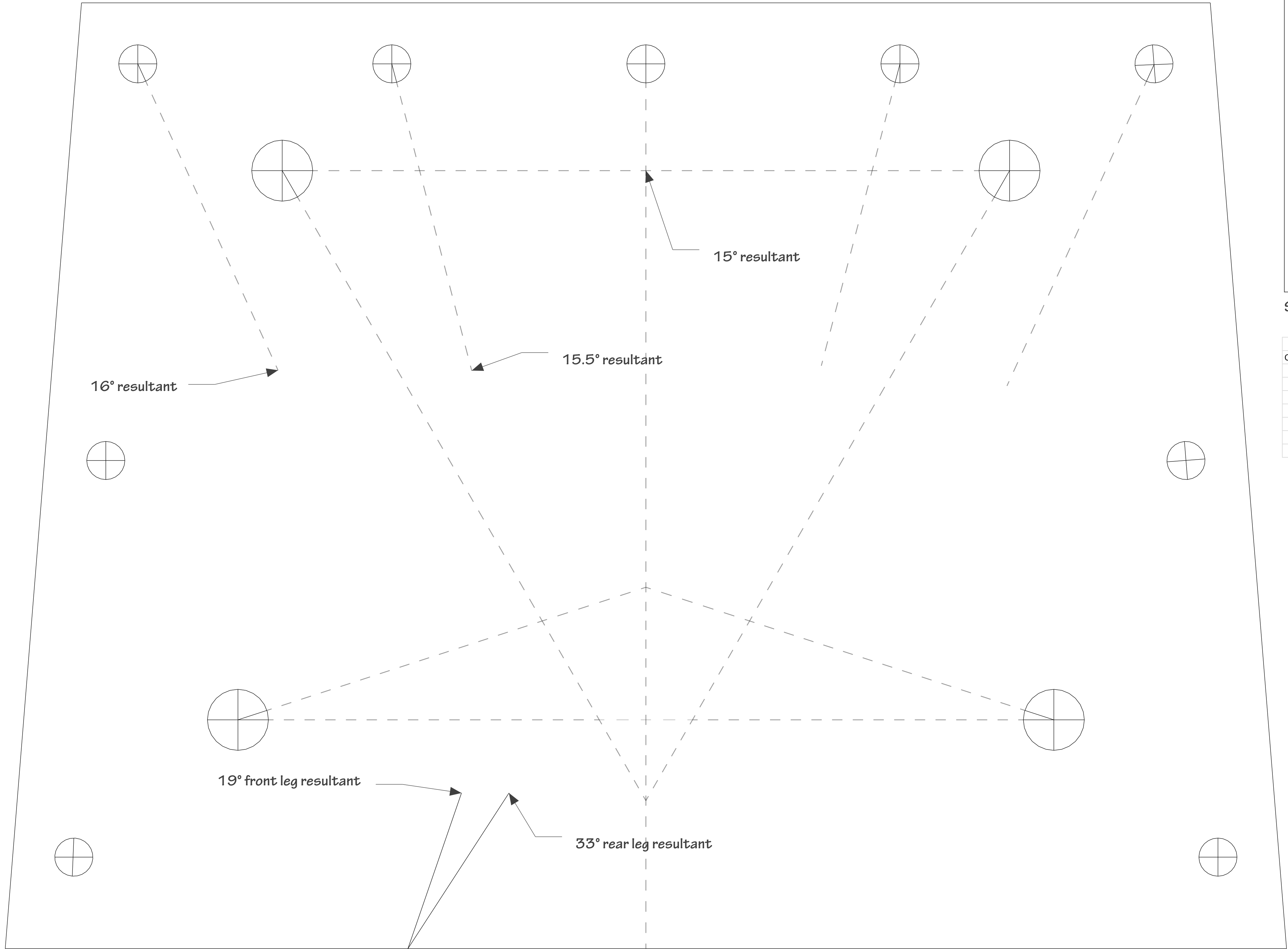
Seat drilling jig, made from 2x material
