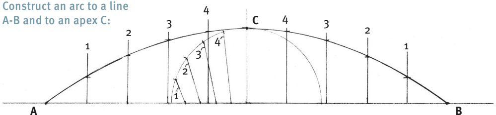
FIG. 3.4.2. Expansion from circle to arc.
