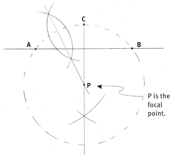
FIG. 3.4.4. Finding an arc's focal point.
