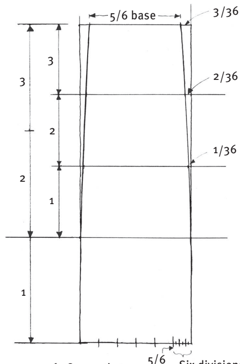
FIG. 3.4.16. Generating an entasis taper. Six divisions (6/36)
