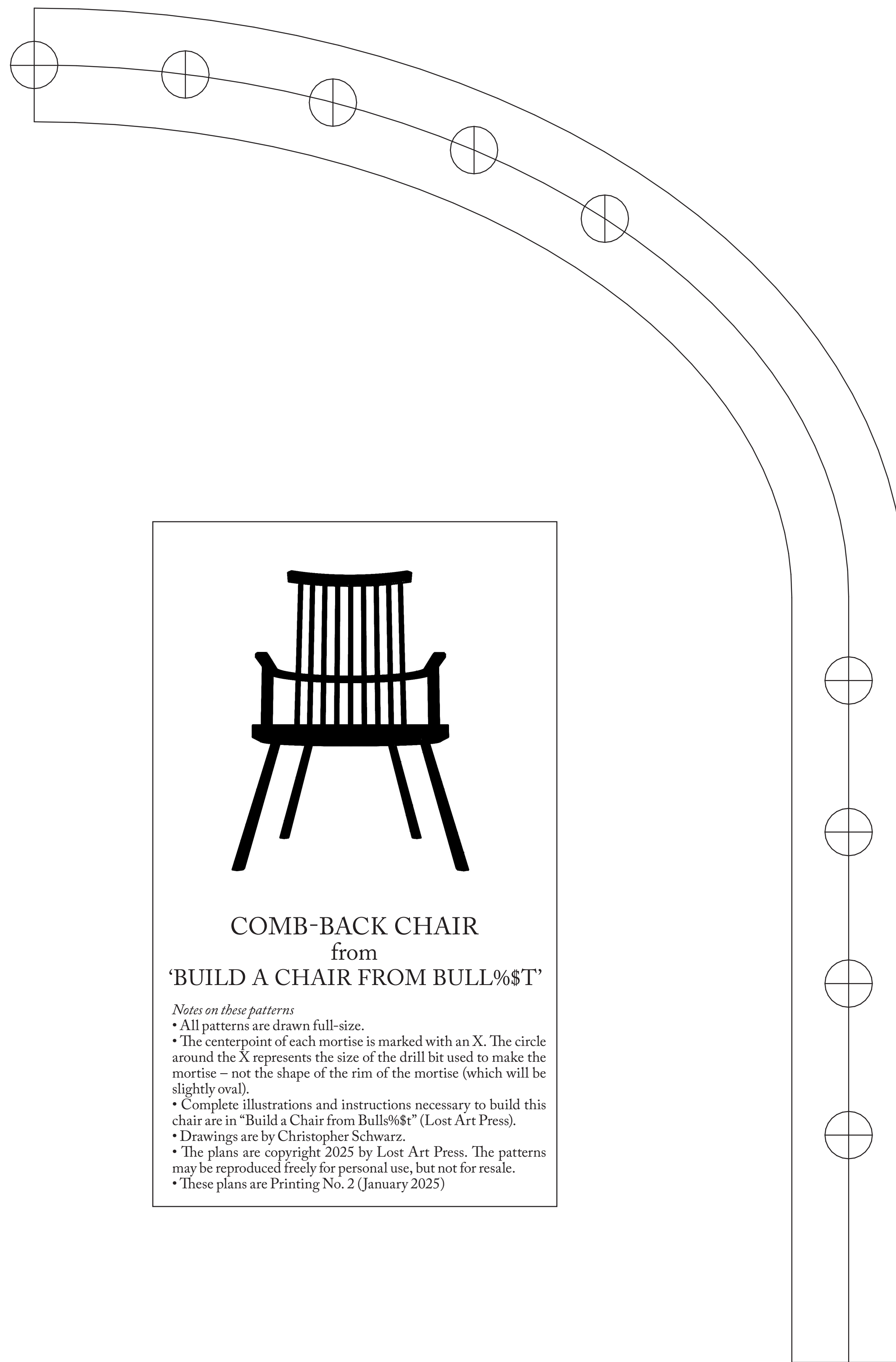
Arm Half-pattern
