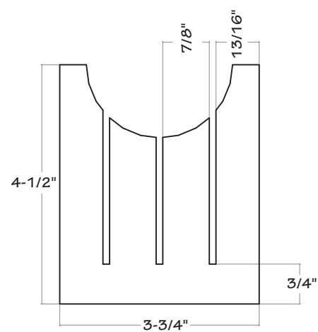
Sawtill detail
