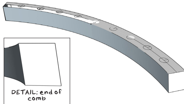
4. Cut front and rear edge of comb at 10 degrees.
