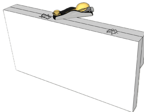
5. Remove high spots with a block plane.
