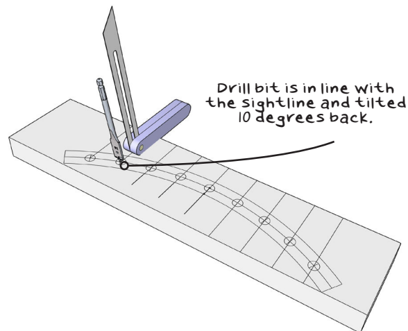
3. Drill mortises into comb at 10 degrees.
