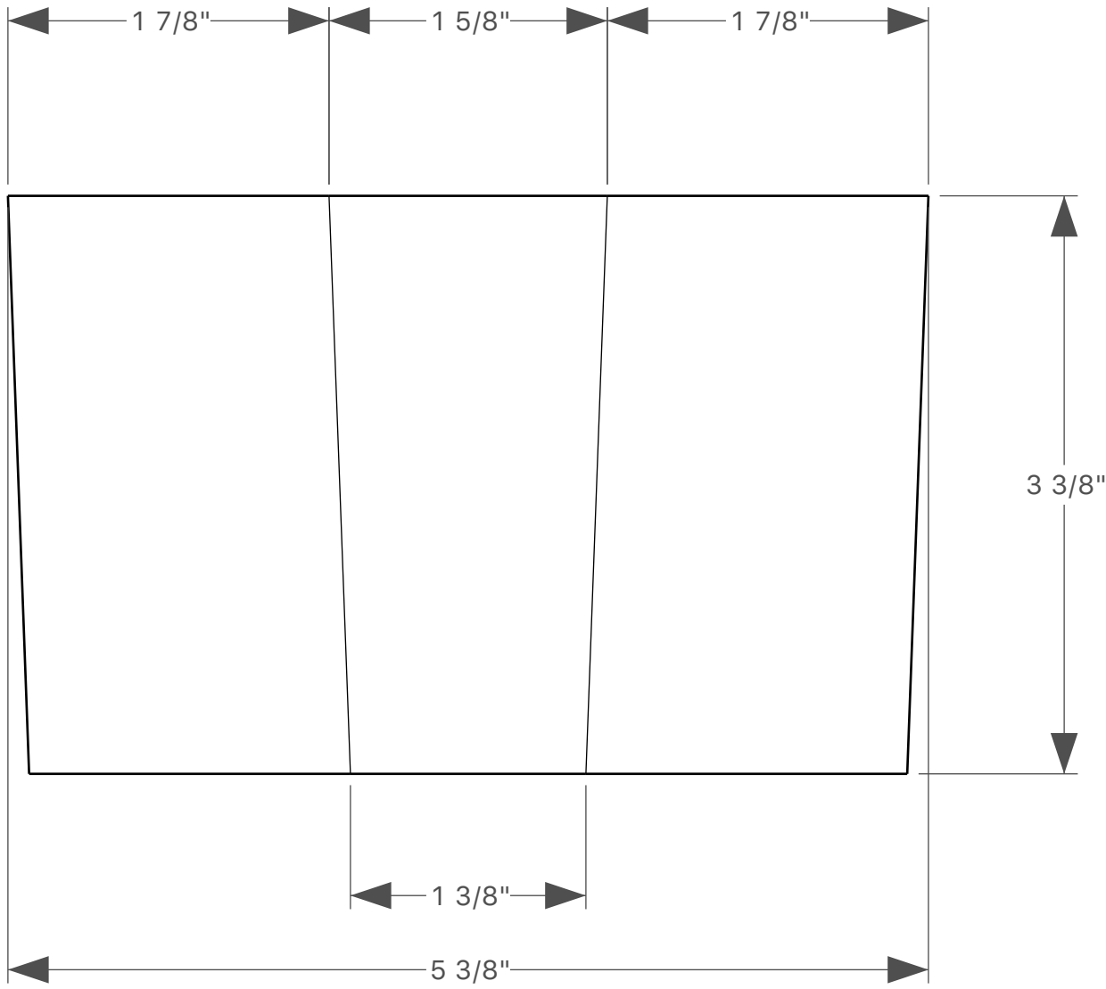
Mallet Head, Elevation
