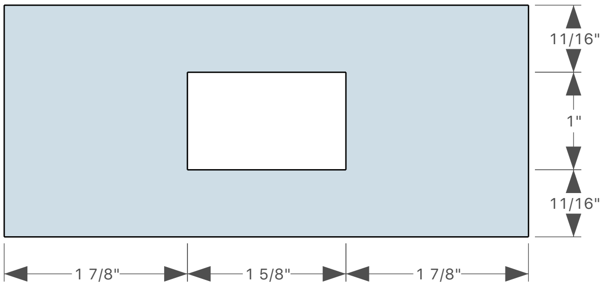
Mallet Head, Top
