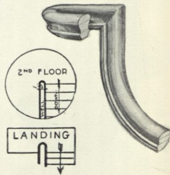
M-743 (1 Riser) M-743A (2 Risers) Goose Neck Landing Return, Left
